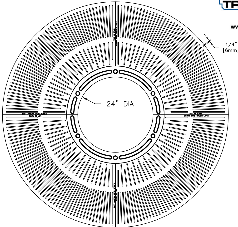
GRATE PLAN VIEW
