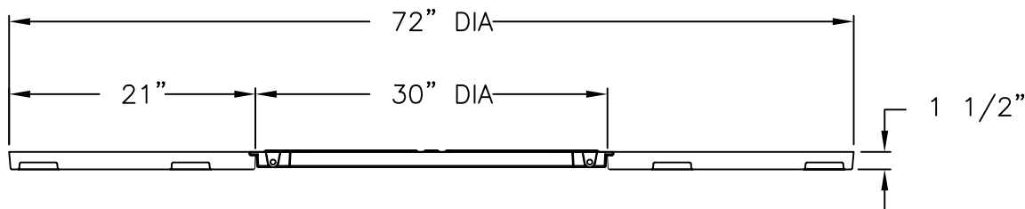
GRATE SECTION VIEW
